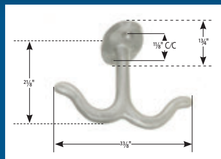
NO. 180 WARDROBE HOOK
