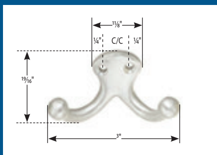
NO. 181 WARDROBE HOOK
