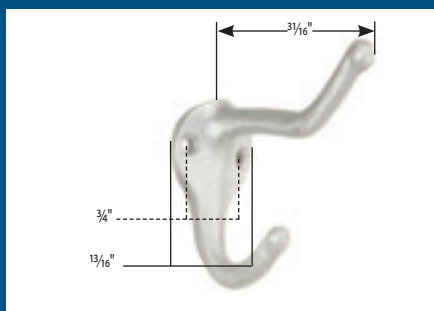
NO. 171 COAT HOOK
