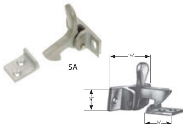
NO. 20-SA ALUMINUM ELBOW CATCH
