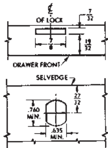
MOUNTING HOLES
