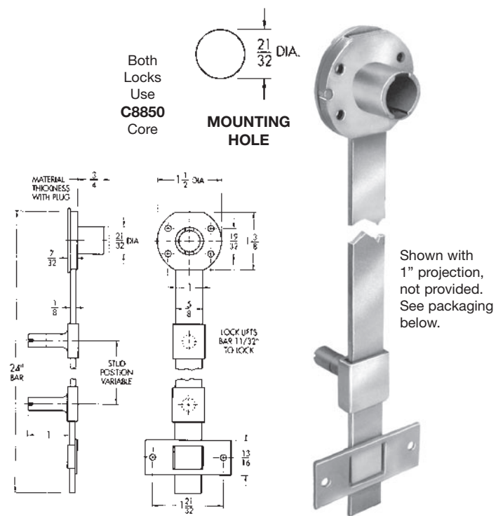
D8840 Side Mounted Gang Lock
