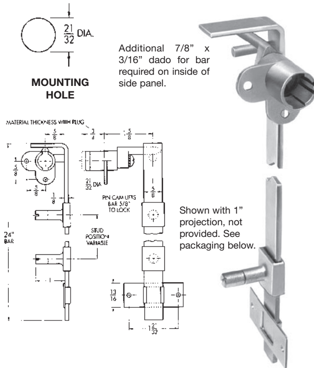
D8838 Front Mounted Gang Lock
