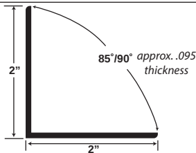
Part # 1755-CL
