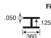
Part # ALU0829-S
