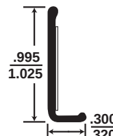
Part # 2001-*
