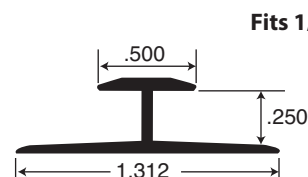
Part # ALU1798-*
