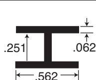
Part # ALU4299-*
