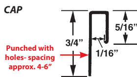
Part # SS1451-P
