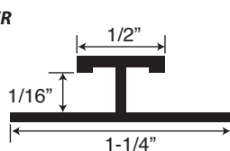
Part # SS1450-P
