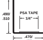
Part # 2407-*
