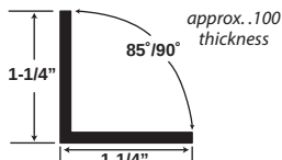
Part # 1750-CL
