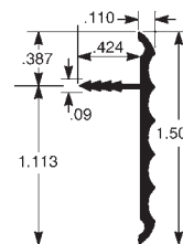
1-1/2" Off-set Barb
