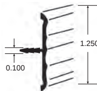
13/16" Center Barb
