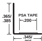
Part # 2406-*
