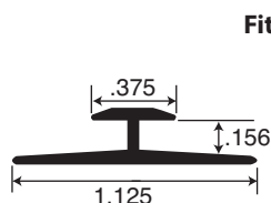
Part # ALU5639-*
