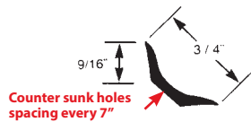
Part # ALU121-PH
