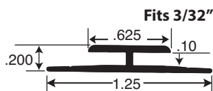
Part # ALU5044-S
