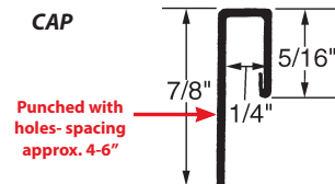
Part # SS851-P
