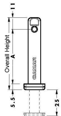
'A' Dimension will change with the height of the leveler - see chart.
