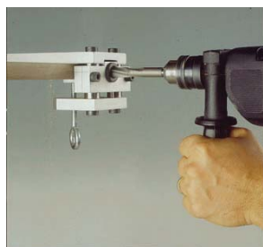
Use the template to drill the placement hole.
