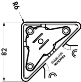
Mounting Bracket
