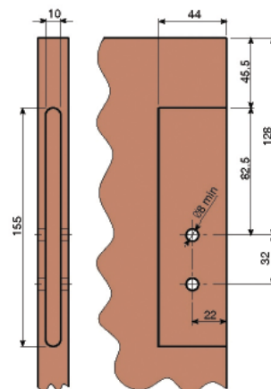
Drilling of the side
