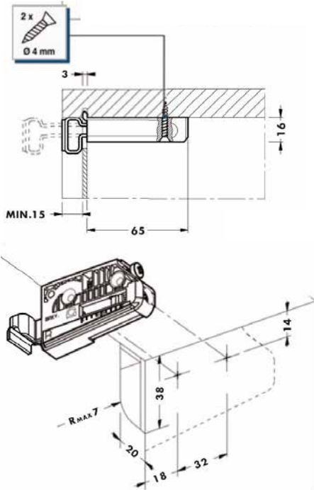
Screw Mount
