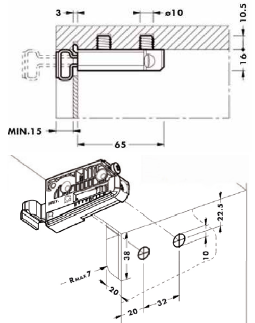
Dowel Mount
