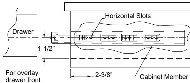
Figure 1 Conventional Mounting—Cabinet
