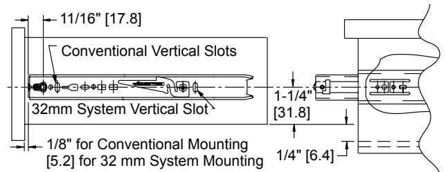
Figure 4 Conventional and 32 mm Mounting—Drawer
